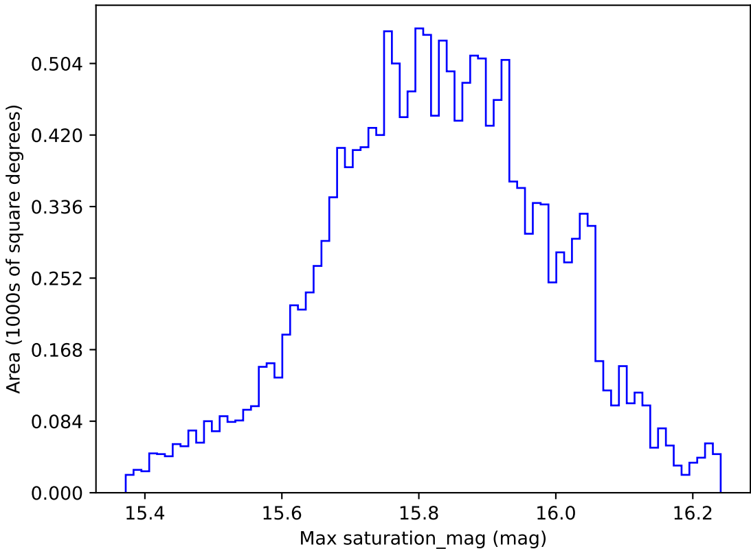
extra_ss_neo3_v3.4_10yrs WFD all bands: Max saturation_mag
