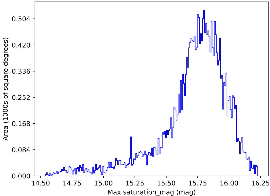
extra_ss_neo3_v3.4_10yrs All sky all bands: Max saturation_mag
