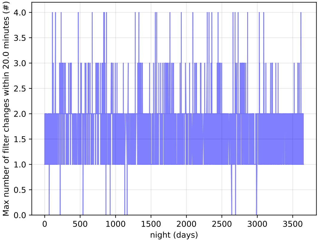
extra_ss_neo3_v3.4_10yrs Per Night: Max number of filter changes within 20.0 minutes
