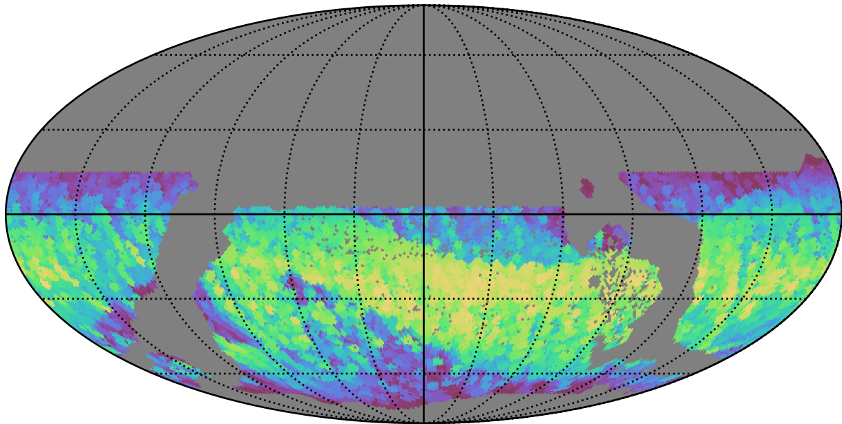
extra_ss_neo3_v3.4_10yrs WFD all bands: Max normairmass
