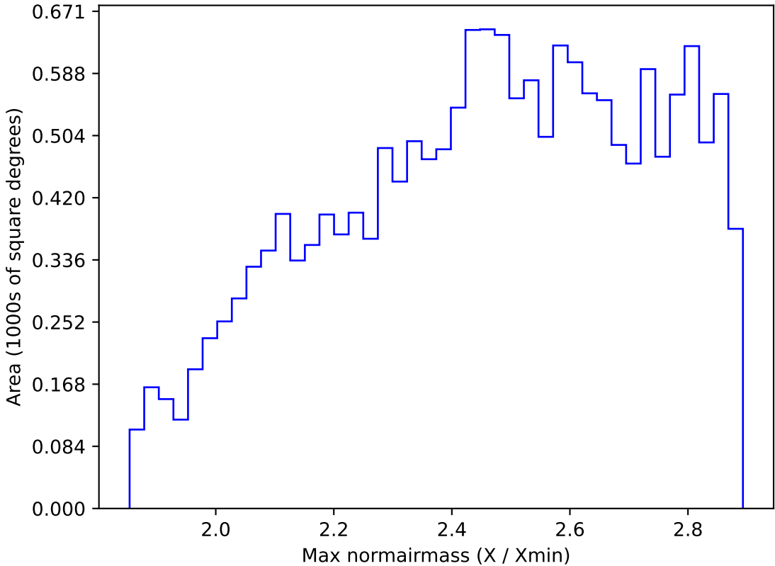
extra_ss_neo3_v3.4_10yrs WFD all bands: Max normairmass
