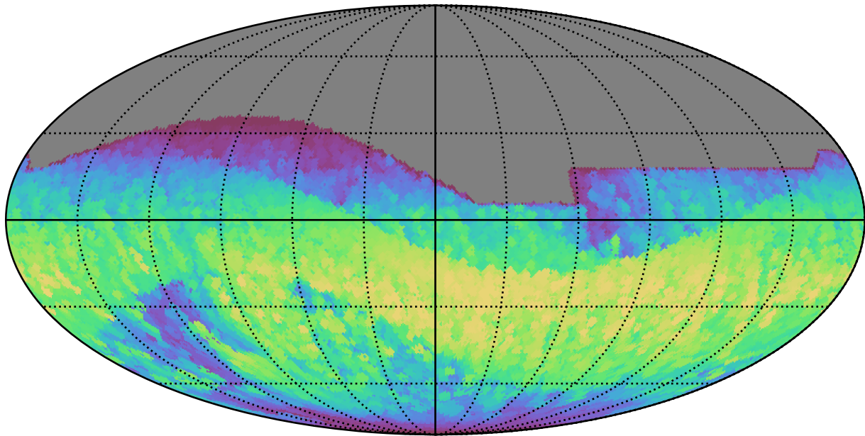
extra_ss_neo3_v3.4_10yrs All sky all bands: Max normairmass
