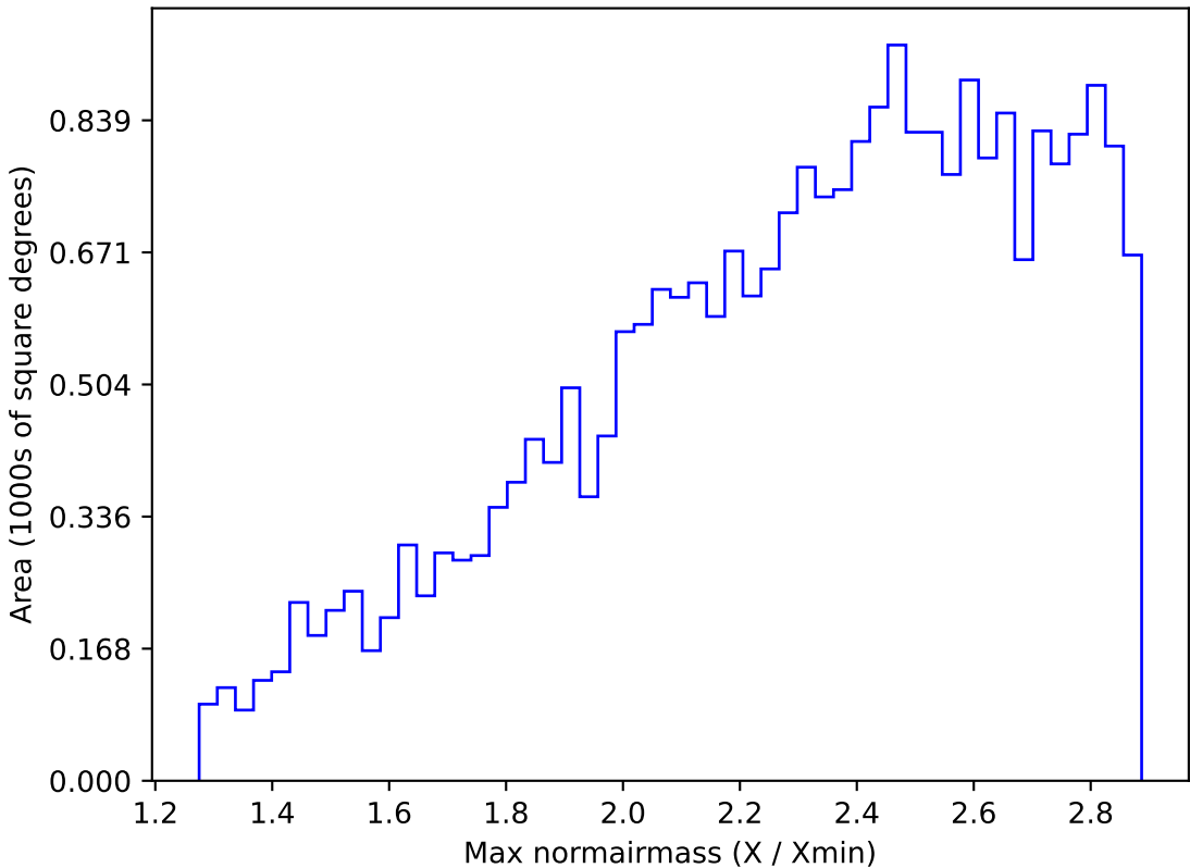
extra_ss_neo3_v3.4_10yrs All sky all bands: Max normairmass
