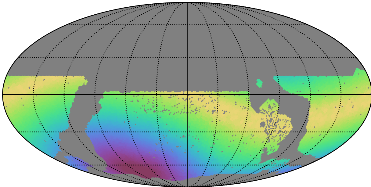
extra_ss_neo3_v3.4_10yrs WFD all bands: Max moonDistance
