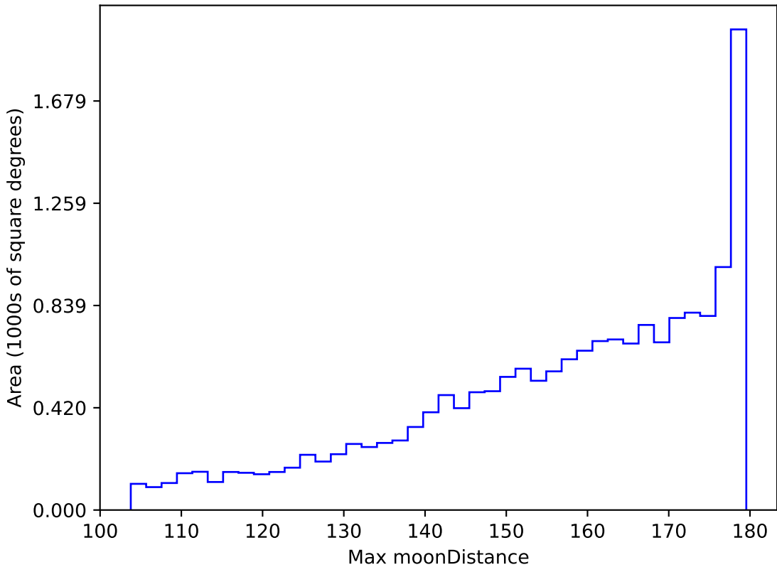
extra_ss_neo3_v3.4_10yrs WFD all bands: Max moonDistance
