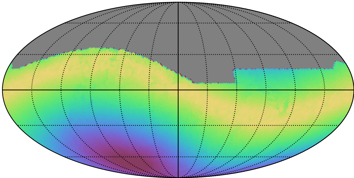
extra_ss_neo3_v3.4_10yrs All sky all bands: Max moonDistance
