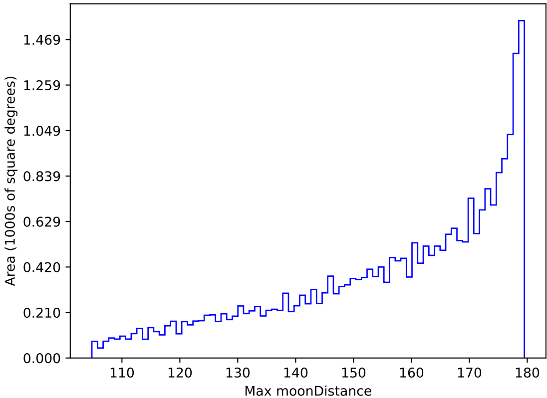
extra_ss_neo3_v3.4_10yrs All sky all bands: Max moonDistance
