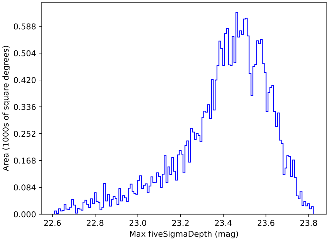
extra_ss_neo3_v3.4_10yrs Yr 1 z band: Max fiveSigmaDepth
