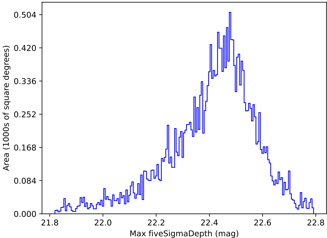
extra_ss_neo3_v3.4_10yrs Yr 1 y band: Max fiveSigmaDepth
