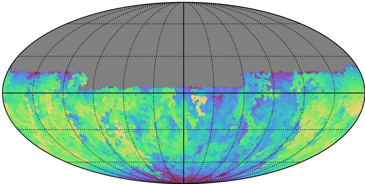
extra_ss_neo3_v3.4_10yrs Yr 1 u band: Max fiveSigmaDepth
