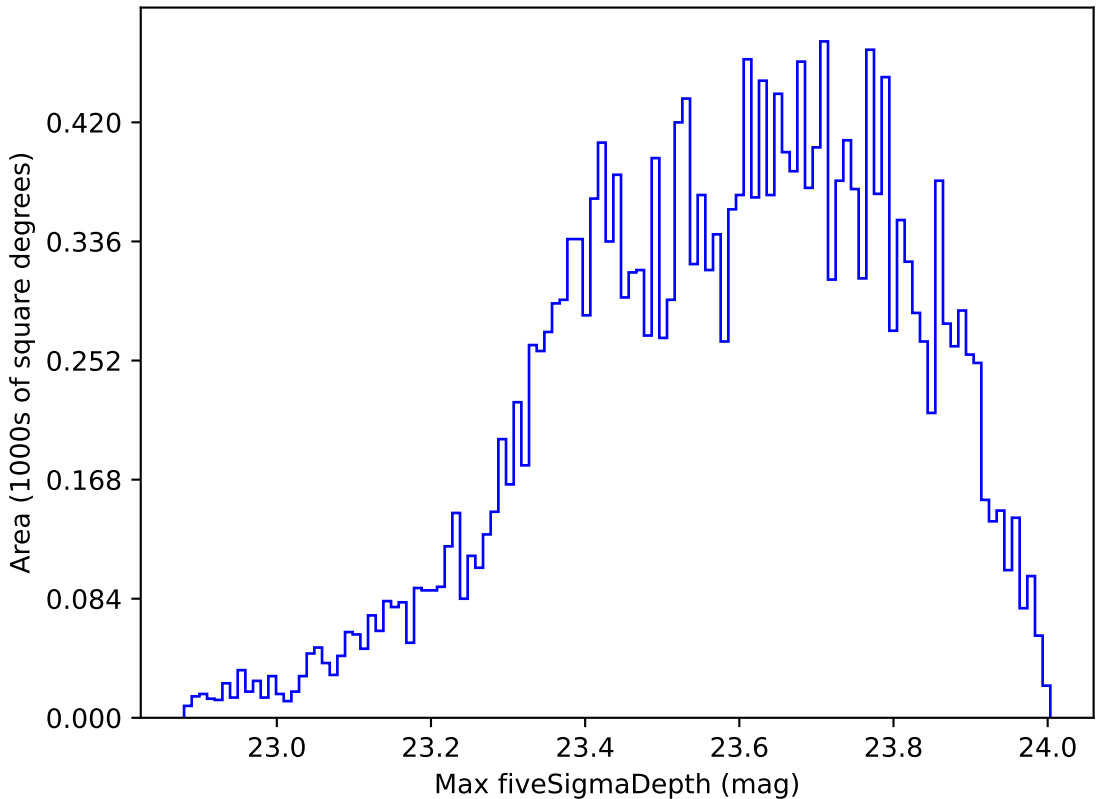
extra_ss_neo3_v3.4_10yrs Yr 1 u band: Max fiveSigmaDepth
