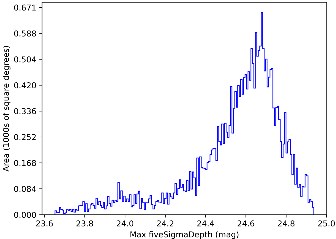
extra_ss_neo3_v3.4_10yrs Yr 1 r band: Max fiveSigmaDepth
