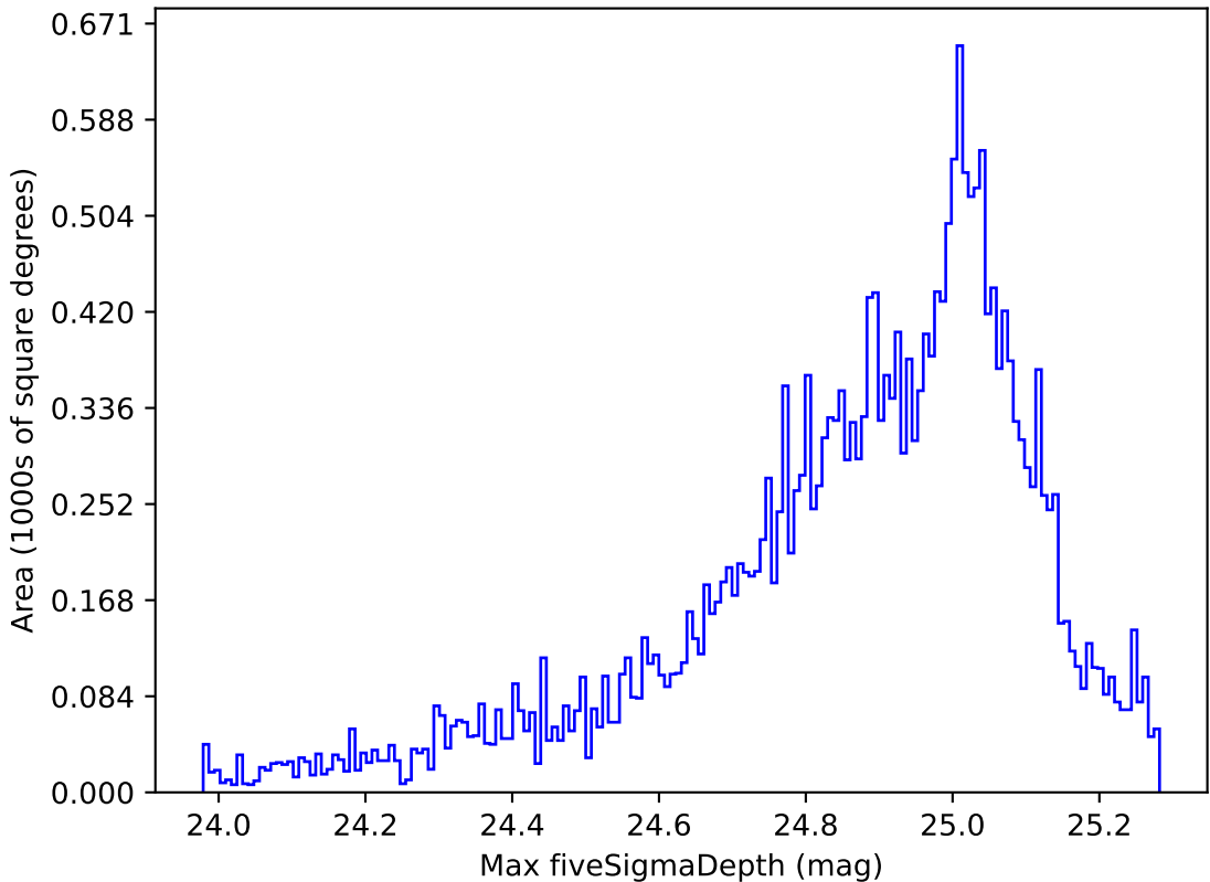
extra_ss_neo3_v3.4_10yrs Yr 1 g band: Max fiveSigmaDepth
