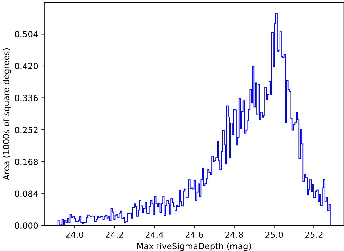
extra_ss_neo3_v3.4_10yrs Yr 1 all bands: Max fiveSigmaDepth
