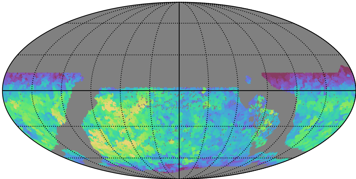
extra_ss_neo3_v3.4_10yrs WFD z band: Max fiveSigmaDepth
