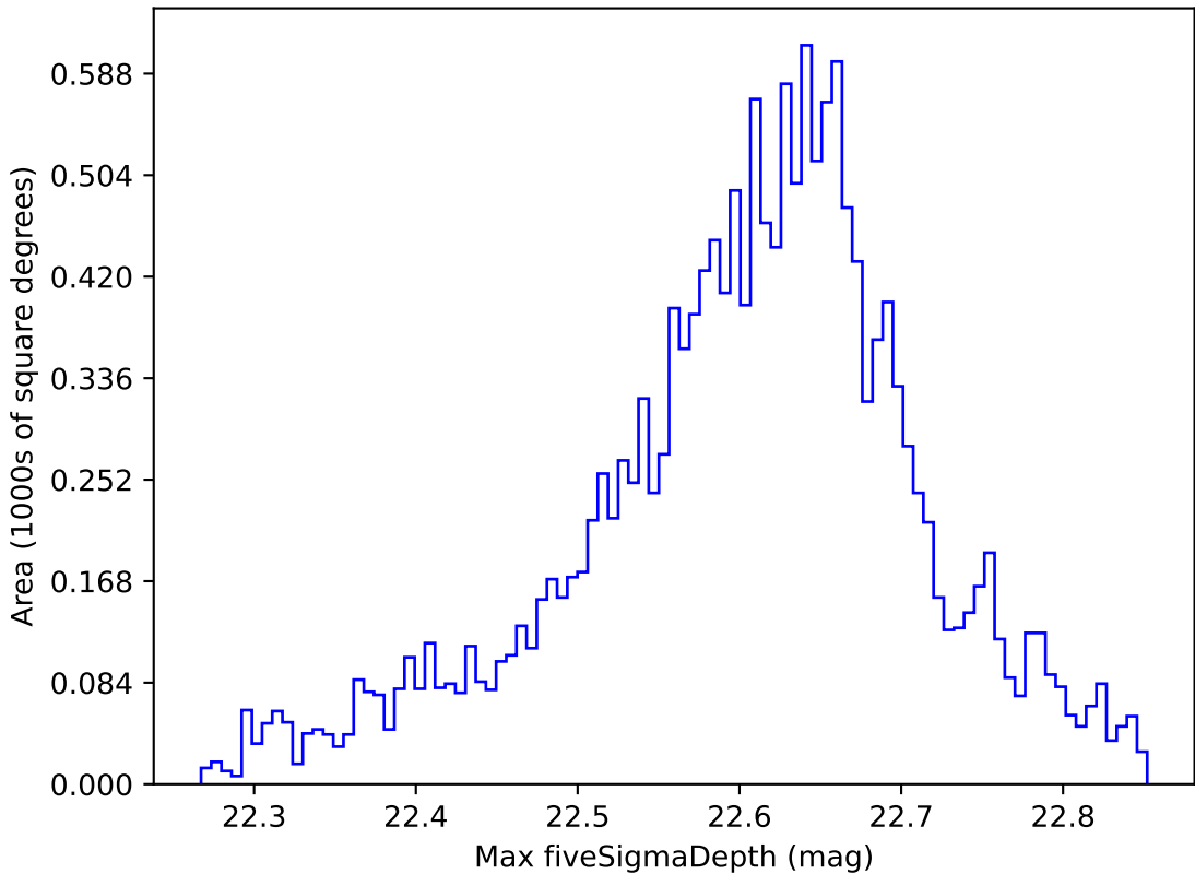
extra_ss_neo3_v3.4_10yrs WFD y band: Max fiveSigmaDepth
