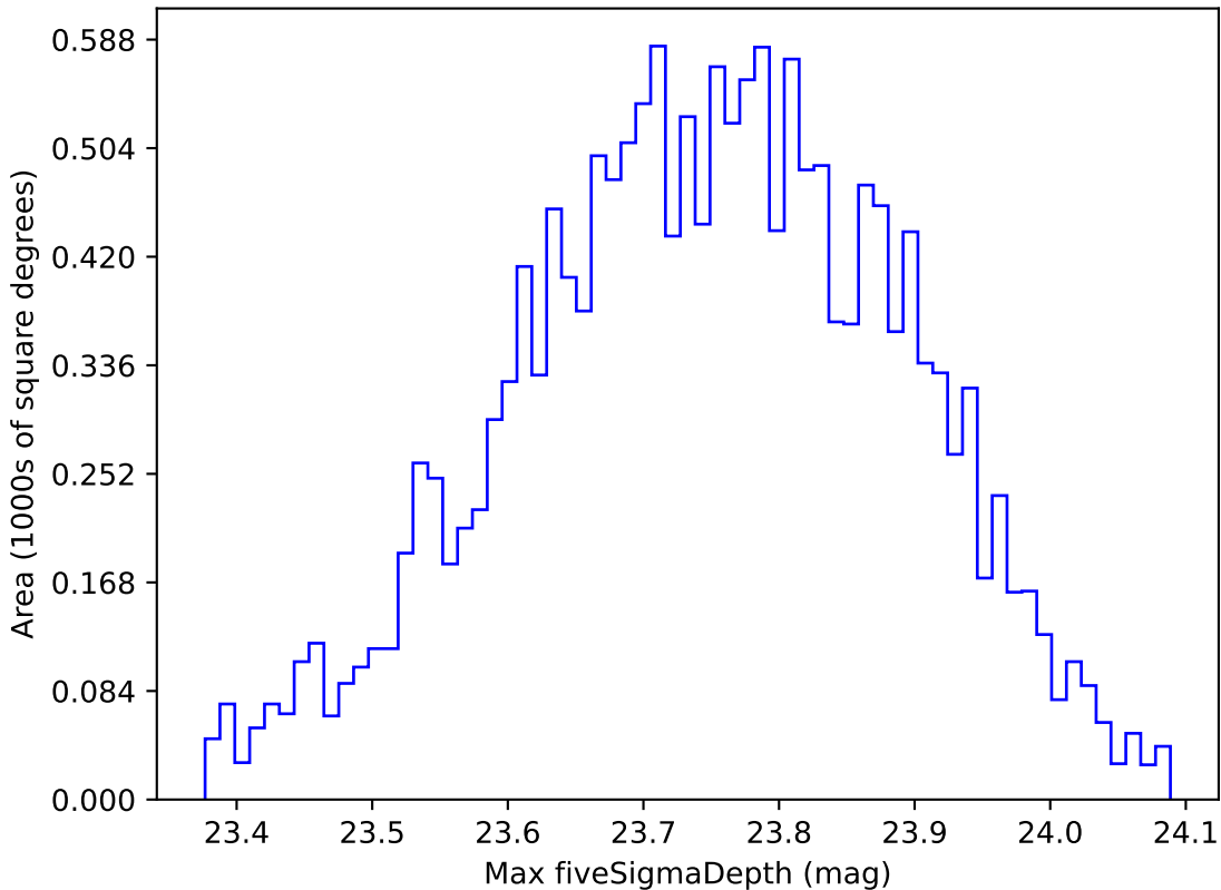
extra_ss_neo3_v3.4_10yrs WFD u band: Max fiveSigmaDepth
