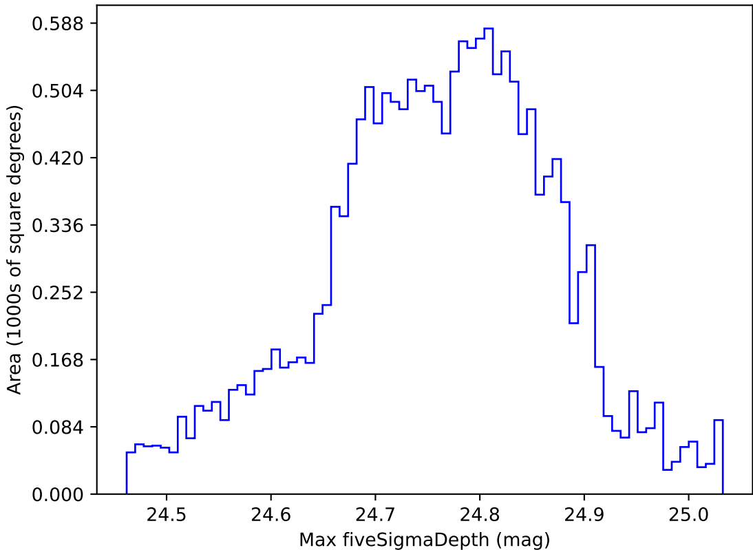
extra_ss_neo3_v3.4_10yrs WFD r band: Max fiveSigmaDepth
