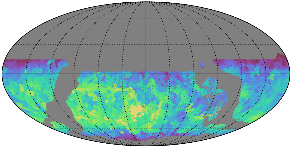
extra_ss_neo3_v3.4_10yrs WFD g band: Max fiveSigmaDepth
