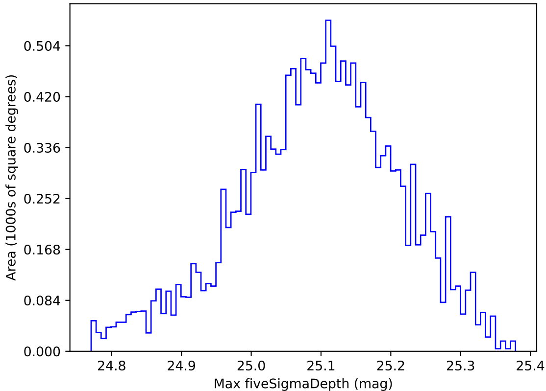
extra_ss_neo3_v3.4_10yrs WFD g band: Max fiveSigmaDepth
