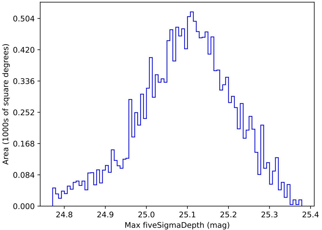
extra_ss_neo3_v3.4_10yrs WFD all bands: Max fiveSigmaDepth
