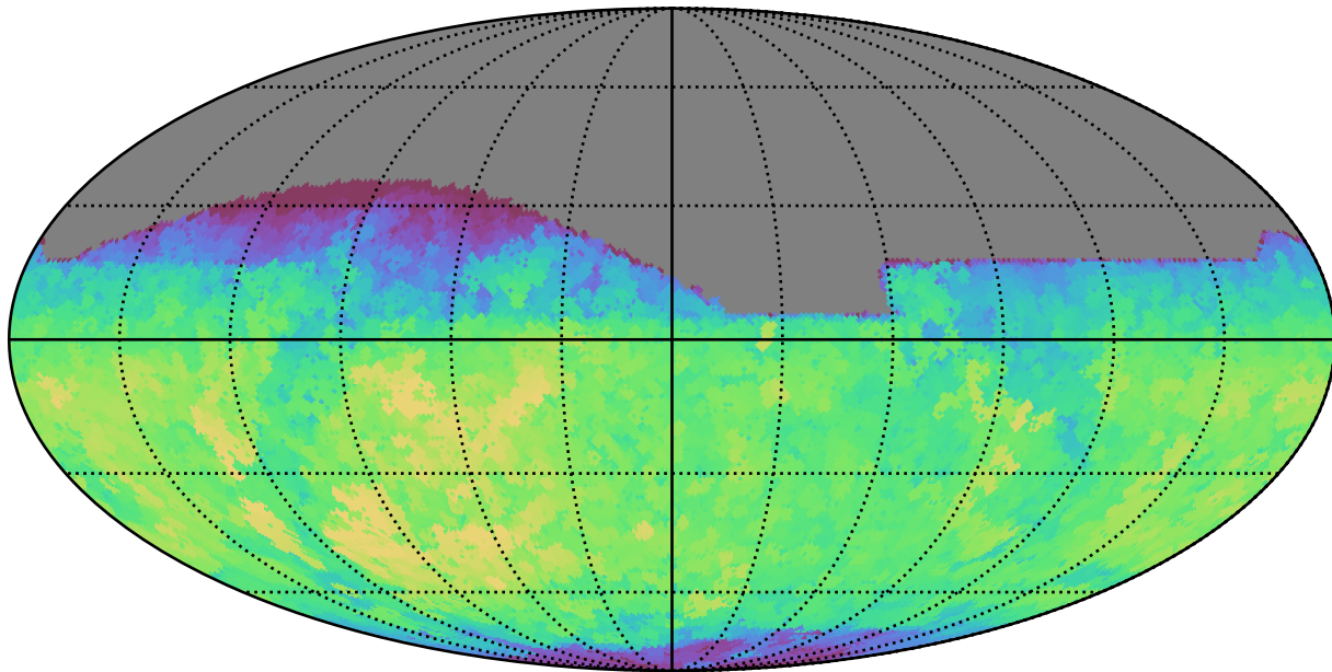
extra_ss_neo3_v3.4_10yrs All sky z band: Max fiveSigmaDepth
