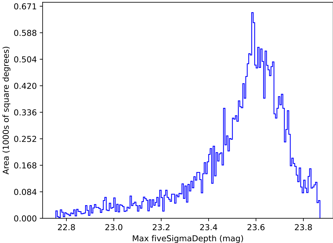
extra_ss_neo3_v3.4_10yrs All sky z band: Max fiveSigmaDepth
