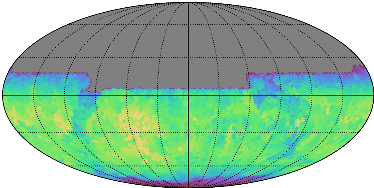
extra_ss_neo3_v3.4_10yrs All sky y band: Max fiveSigmaDepth
