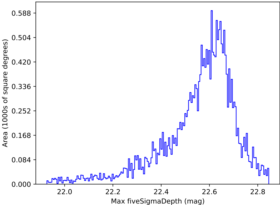
extra_ss_neo3_v3.4_10yrs All sky y band: Max fiveSigmaDepth
