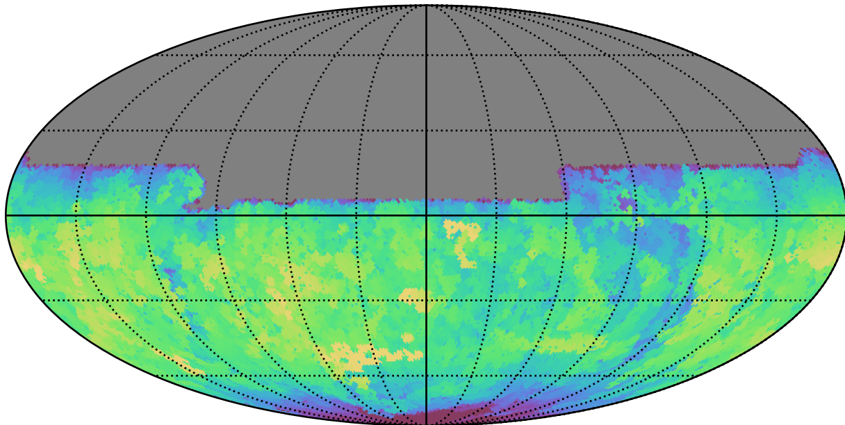
extra_ss_neo3_v3.4_10yrs All sky u band: Max fiveSigmaDepth
