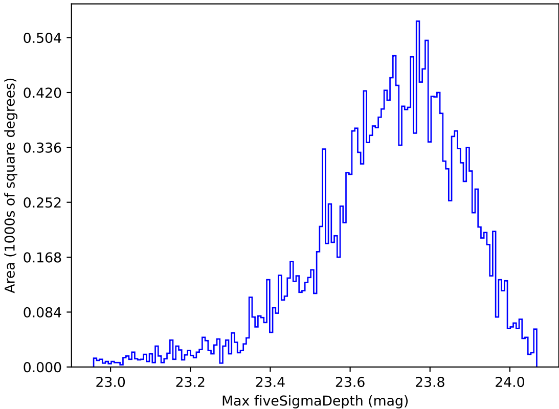
extra_ss_neo3_v3.4_10yrs All sky u band: Max fiveSigmaDepth
