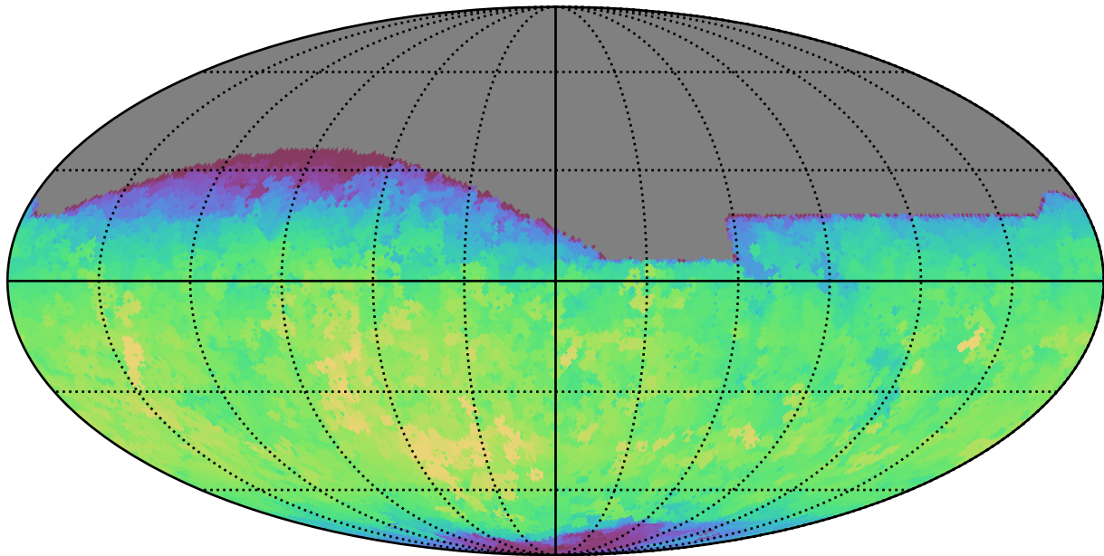
extra_ss_neo3_v3.4_10yrs All sky r band: Max fiveSigmaDepth
