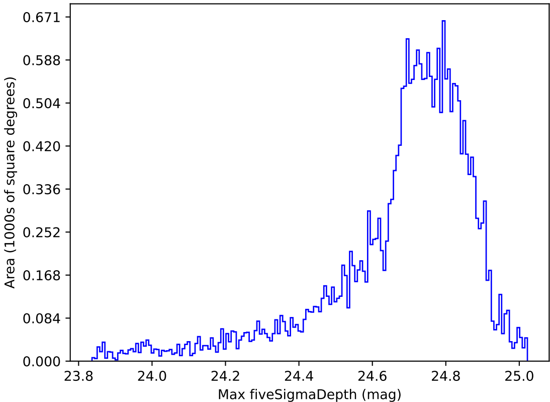
extra_ss_neo3_v3.4_10yrs All sky r band: Max fiveSigmaDepth
