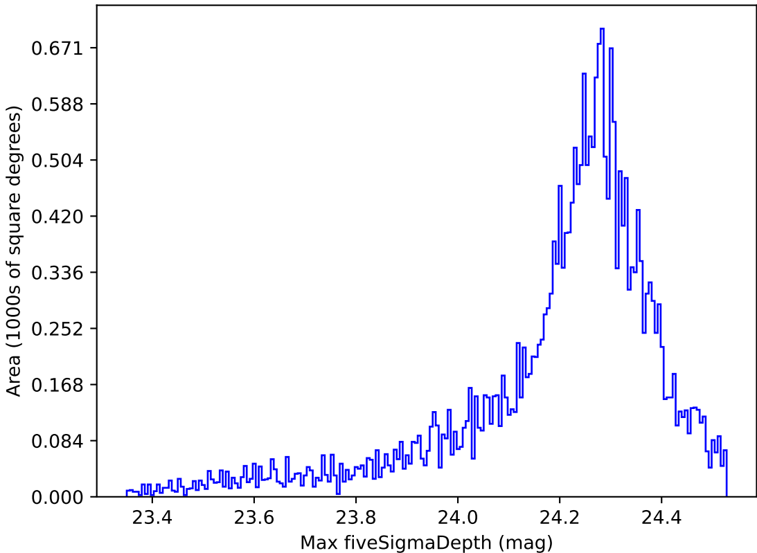
extra_ss_neo3_v3.4_10yrs All sky i band: Max fiveSigmaDepth
