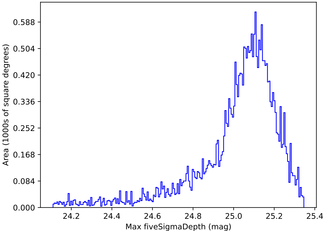
extra_ss_neo3_v3.4_10yrs All sky g band: Max fiveSigmaDepth
