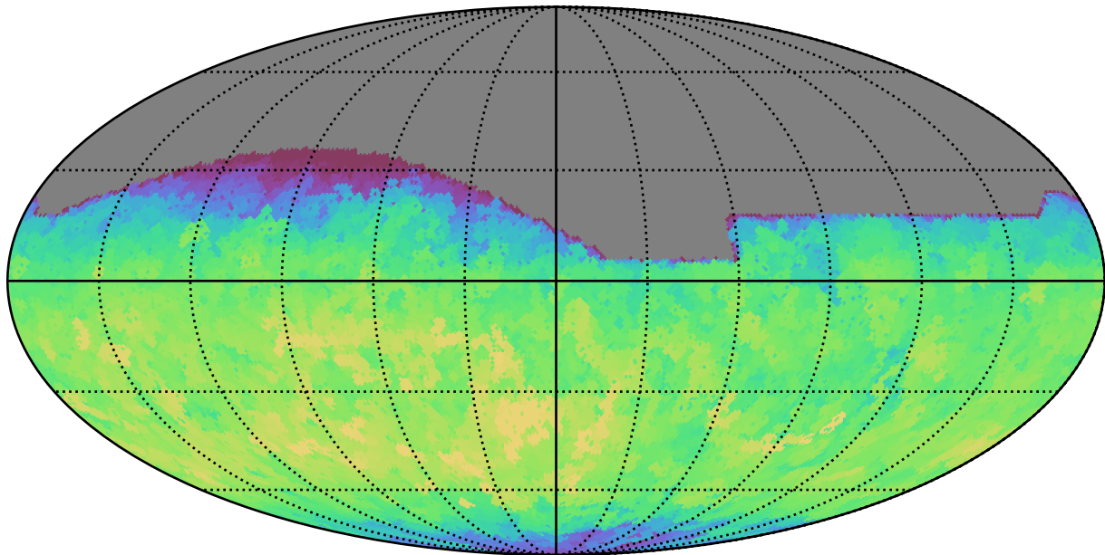
extra_ss_neo3_v3.4_10yrs All sky all bands: Max fiveSigmaDepth
