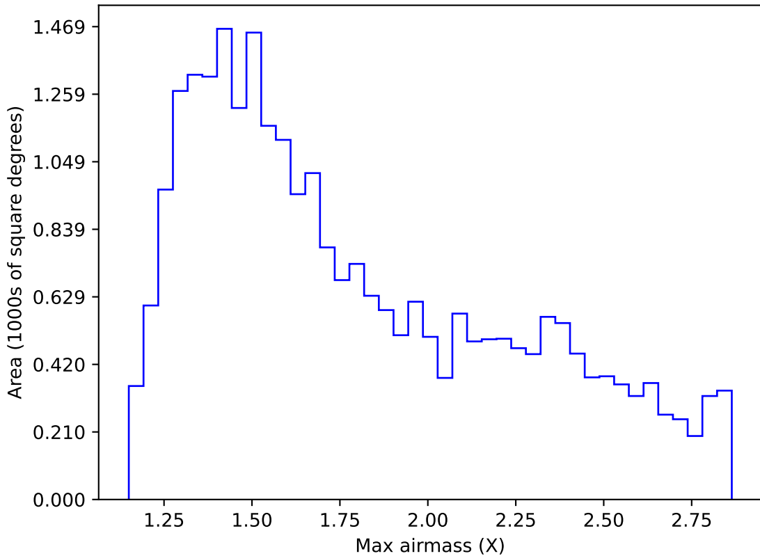
extra_ss_neo3_v3.4_10yrs Yr 1 z band: Max airmass
