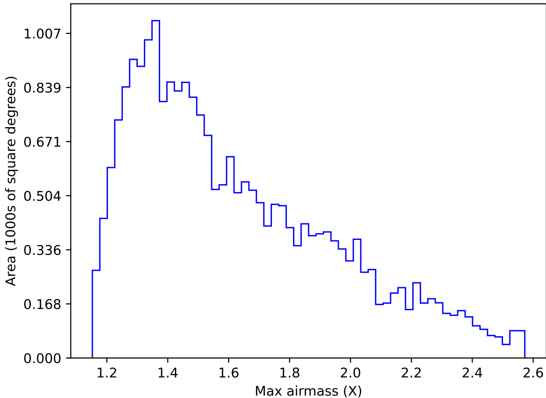
extra_ss_neo3_v3.4_10yrs Yr 1 y band: Max airmass
