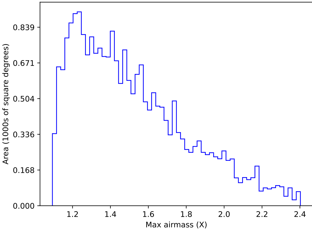
extra_ss_neo3_v3.4_10yrs Yr 1 u band: Max airmass
