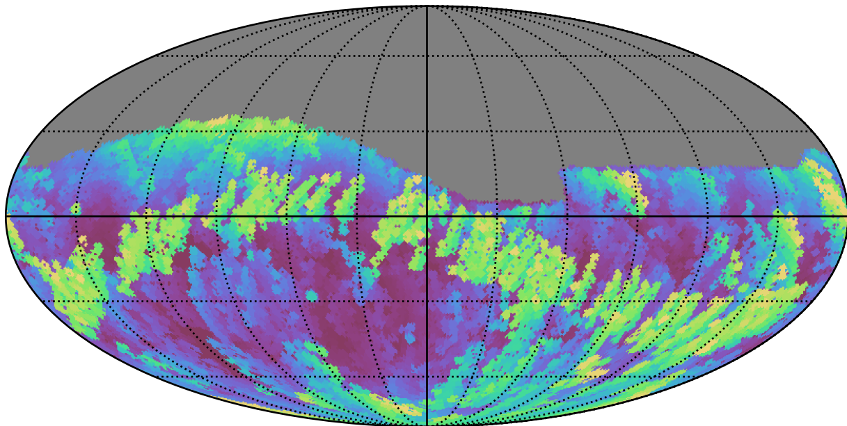
extra_ss_neo3_v3.4_10yrs Yr 1 r band: Max airmass
