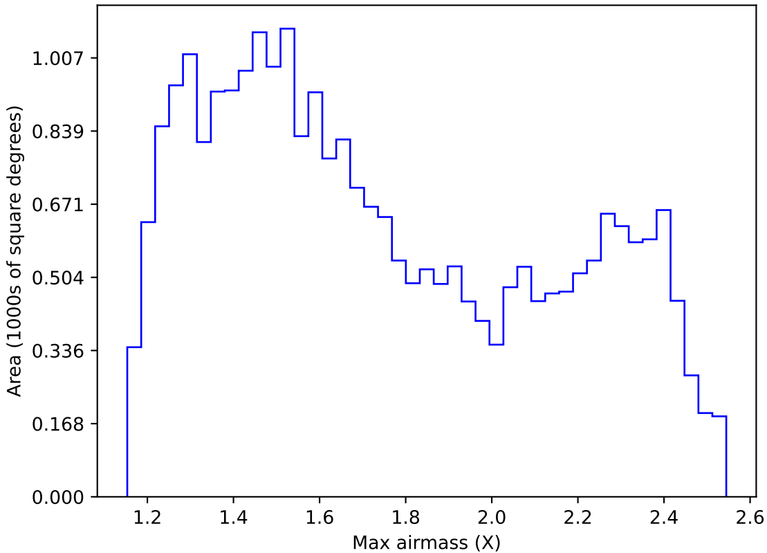
extra_ss_neo3_v3.4_10yrs Yr 1 r band: Max airmass
