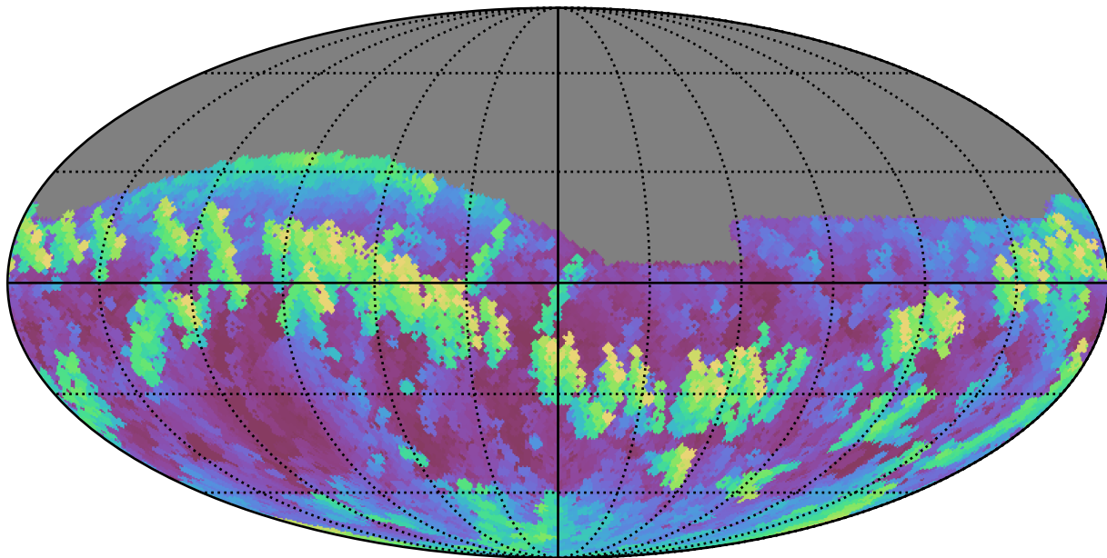
extra_ss_neo3_v3.4_10yrs Yr 1 i band: Max airmass
