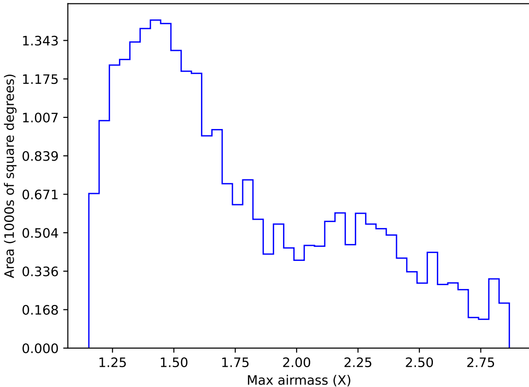
extra_ss_neo3_v3.4_10yrs Yr 1 i band: Max airmass
