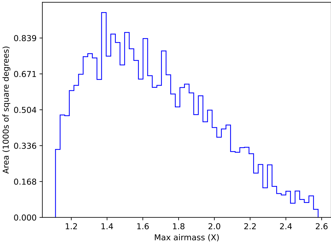
extra_ss_neo3_v3.4_10yrs Yr 1 g band: Max airmass
