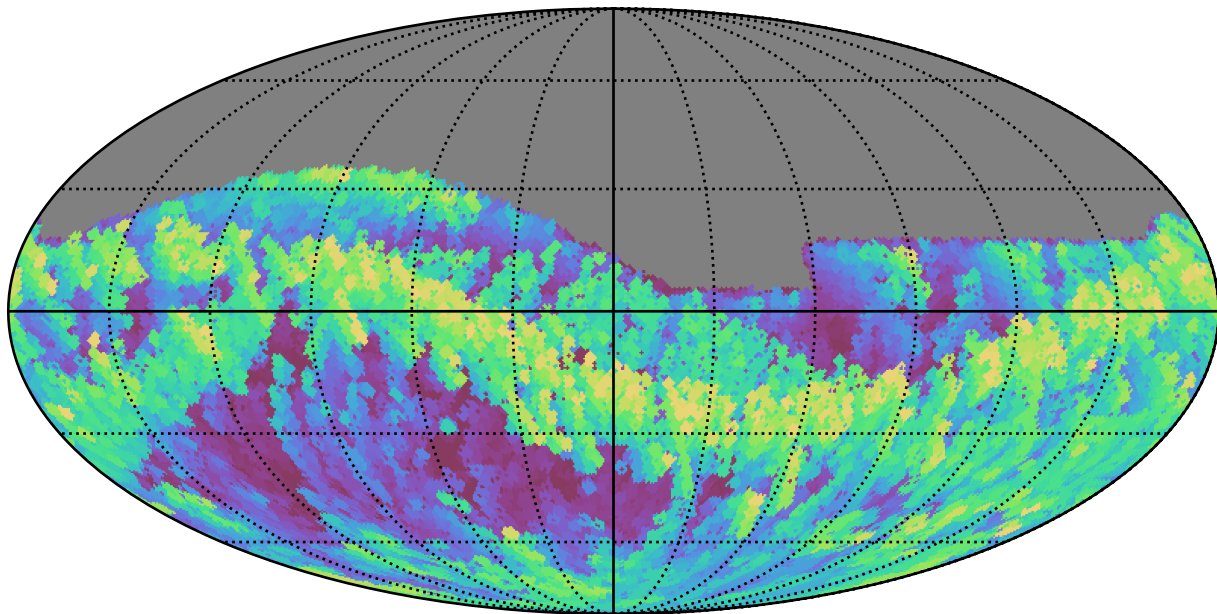
extra_ss_neo3_v3.4_10yrs Yr 1 all bands: Max airmass
