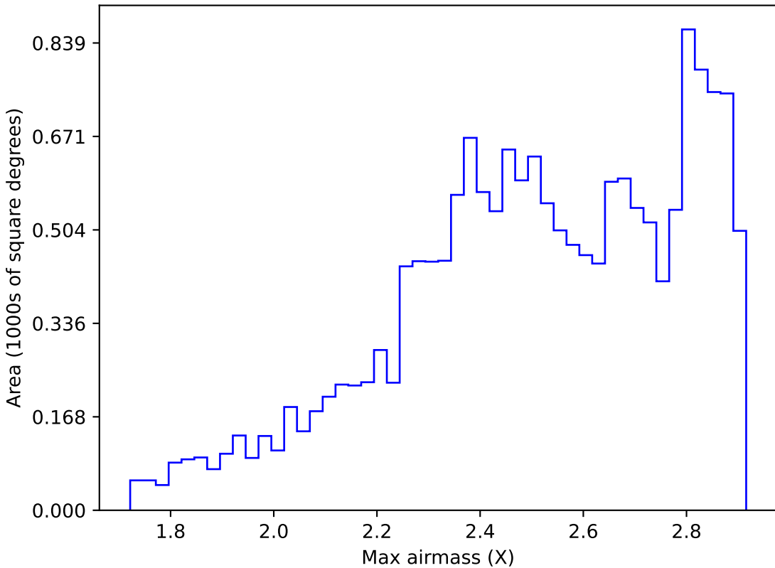
extra_ss_neo3_v3.4_10yrs WFD z band: Max airmass
