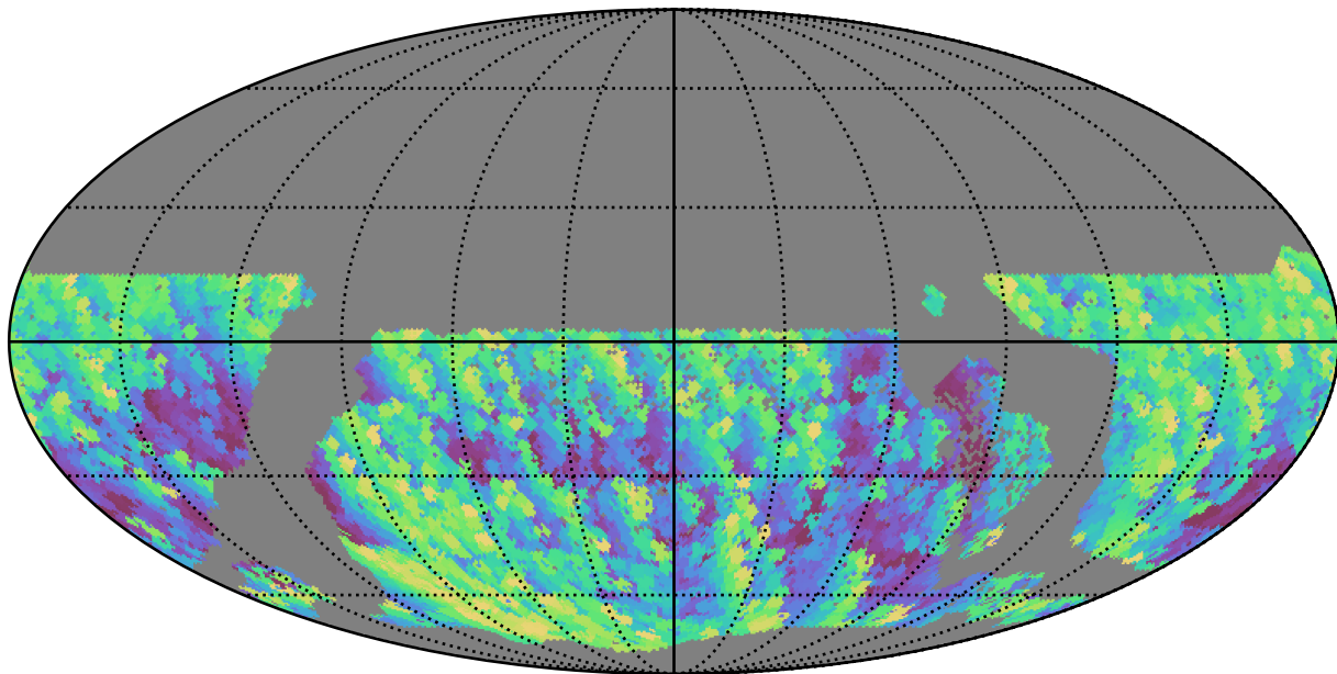
extra_ss_neo3_v3.4_10yrs WFD y band: Max airmass
