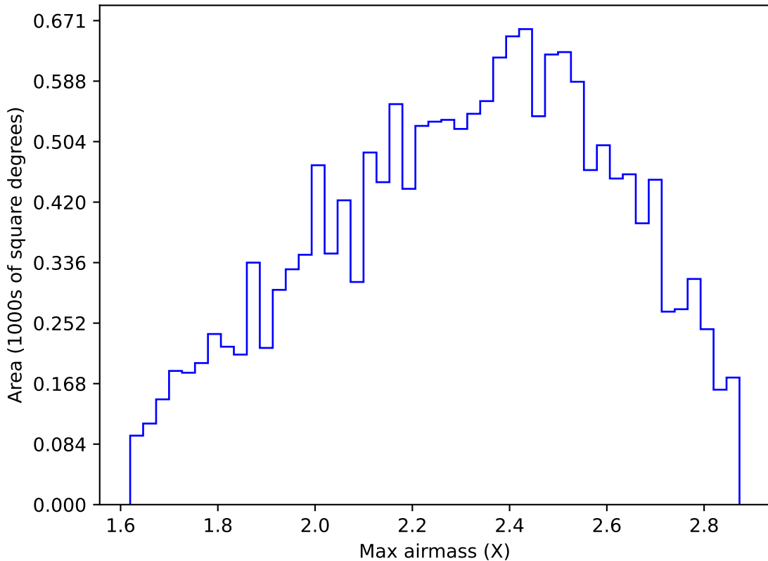
extra_ss_neo3_v3.4_10yrs WFD y band: Max airmass
