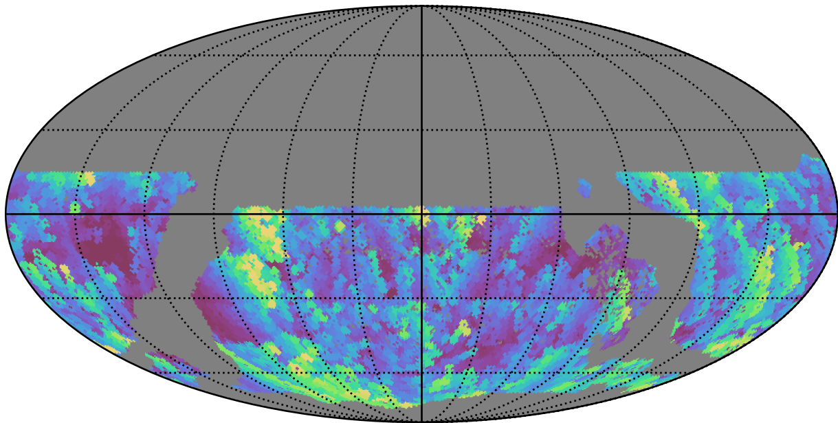
extra_ss_neo3_v3.4_10yrs WFD u band: Max airmass
