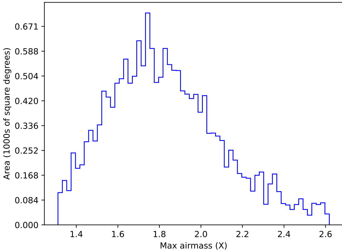
extra_ss_neo3_v3.4_10yrs WFD u band: Max airmass
